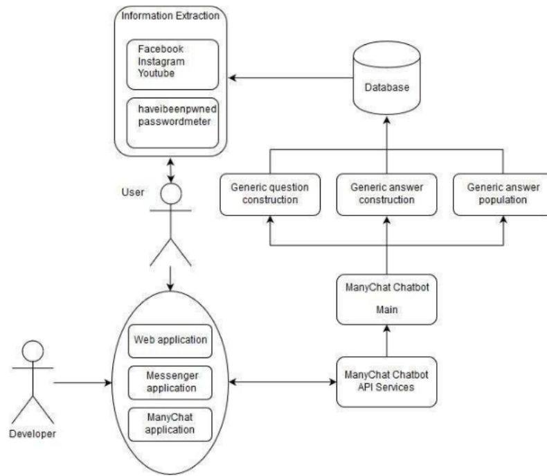
Figure 1: Usecase daigram 1
