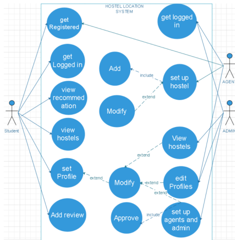
Figure 4: usecase diagram
