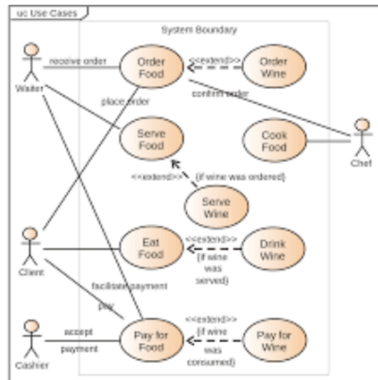
Figure 3: Usecase daigram 2
